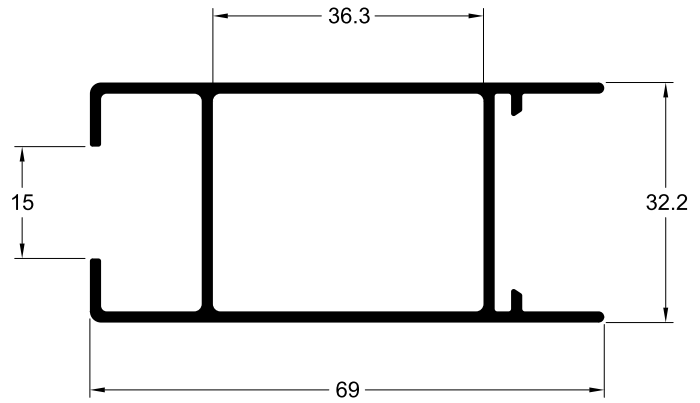
LG-50SB 0,878 Kg/m
