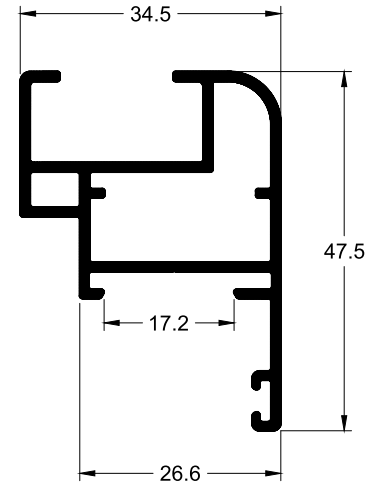
AG-012SB 0.550 Kg/m
