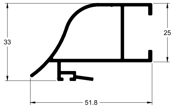
AG-012SB 0.550 Kg/m
