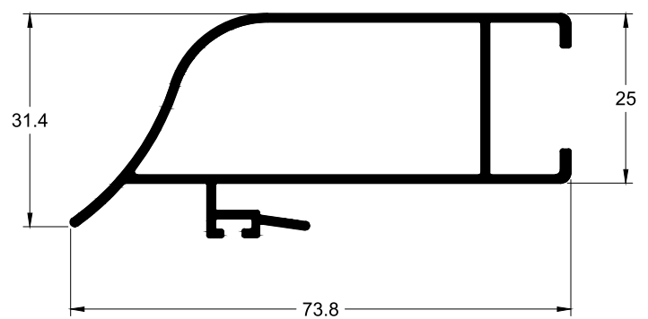
AG-033SB 0.693 Kg/m
