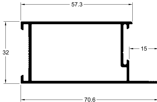
TLG-043S 0.768 Kg/m
