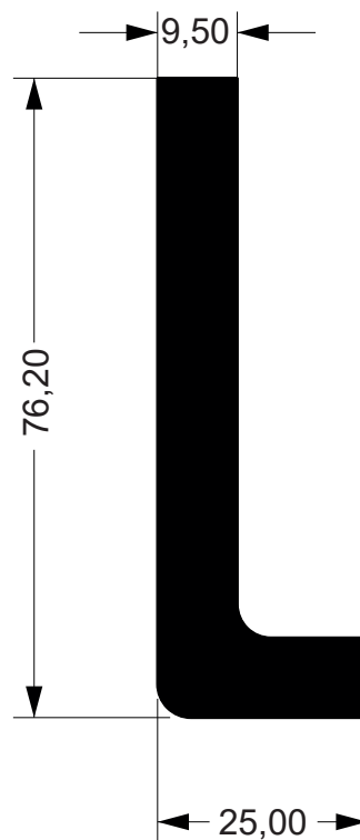
TA-0050 2,360 kg/m
